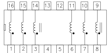
Schematic Diagram
